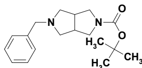
tert-butyl 5-benzyl-octahydropyrrolo[3,4-c]pyrrole-2-carboxylate
