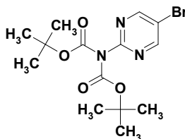
tert-butyl N-(5-bromopyrimidin-2-yl)-N-[(tert-butoxy)carbonyl]carbamate
