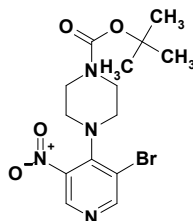
tert-butyl 4-(3-bromo-5-nitropyridin-4-yl)piperazine-1-carboxylate
