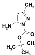
tert-butyl 5-amino-3-methyl-1H-pyrazole-1-carboxylate
