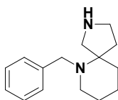
6-benzyl-2,6-diazaspiro[4.5]decane
