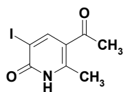
5-acetyl-3-iodo-6-methyl-1,2-dihydropyridin-2-one
