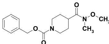
benzyl 4-[methoxy(methyl)carbamoyl]piperidine-1-carboxylate
